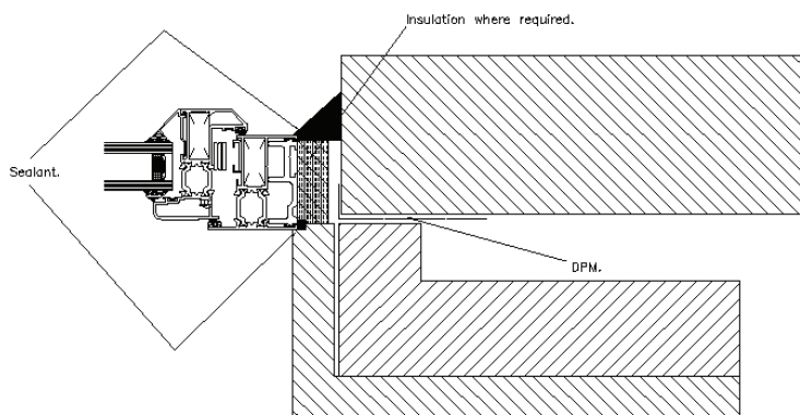
Frame forward of DPM
